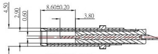
MATE PLUG \phi 4.50
